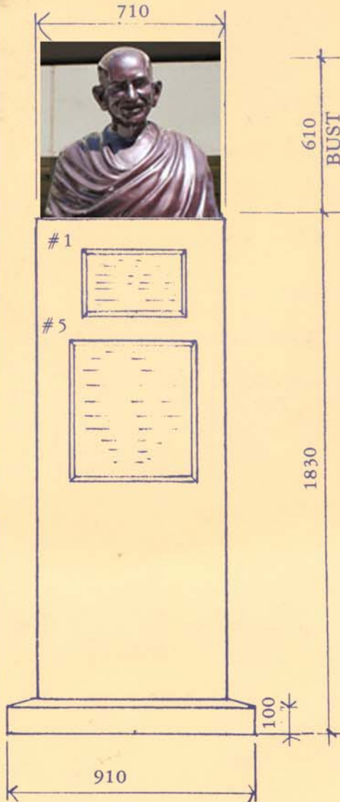
FRONT ELEVATION
